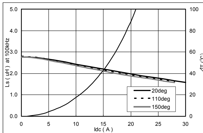
CDMC10D50T150NP-4R3M
