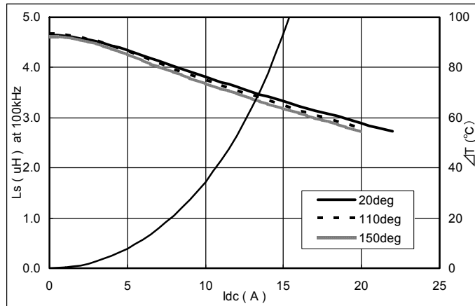
CDMC10D50T150NP-4R3M
